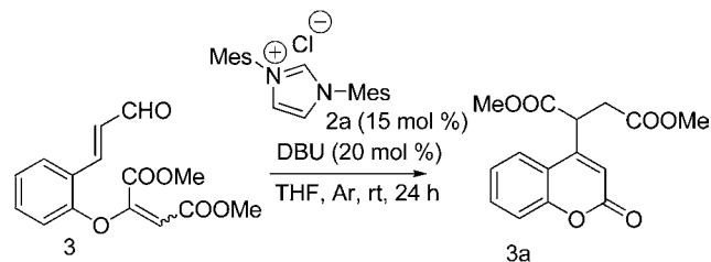
Scheme 2. Proof of the Concept
